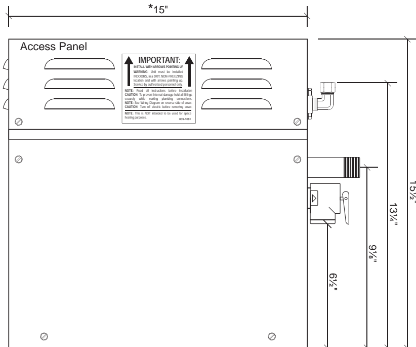
Front Access
